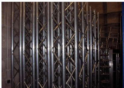
KIT STRUCTURE EUROTRUSS FD34
