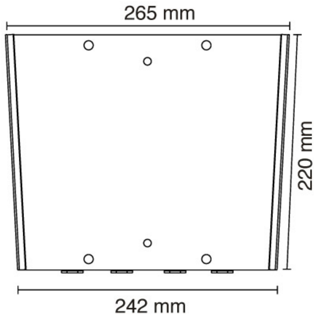
Wall mount
